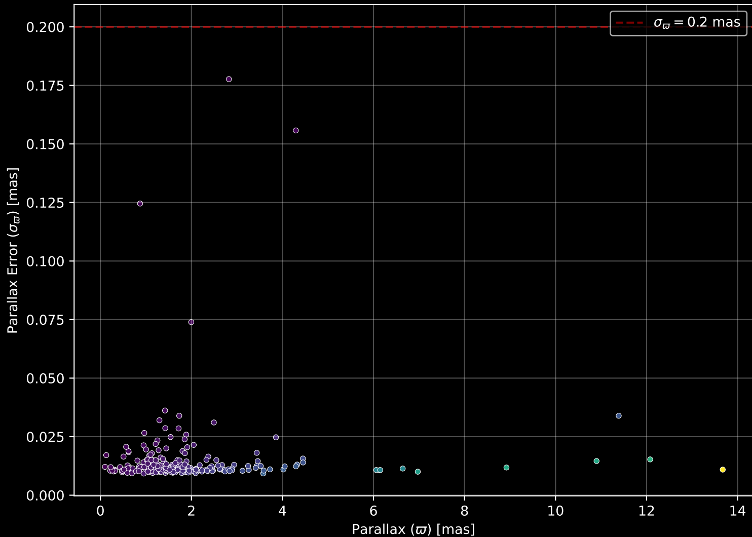
GALAH DR4 Field: [542] Parallax Quality (n= 267)
