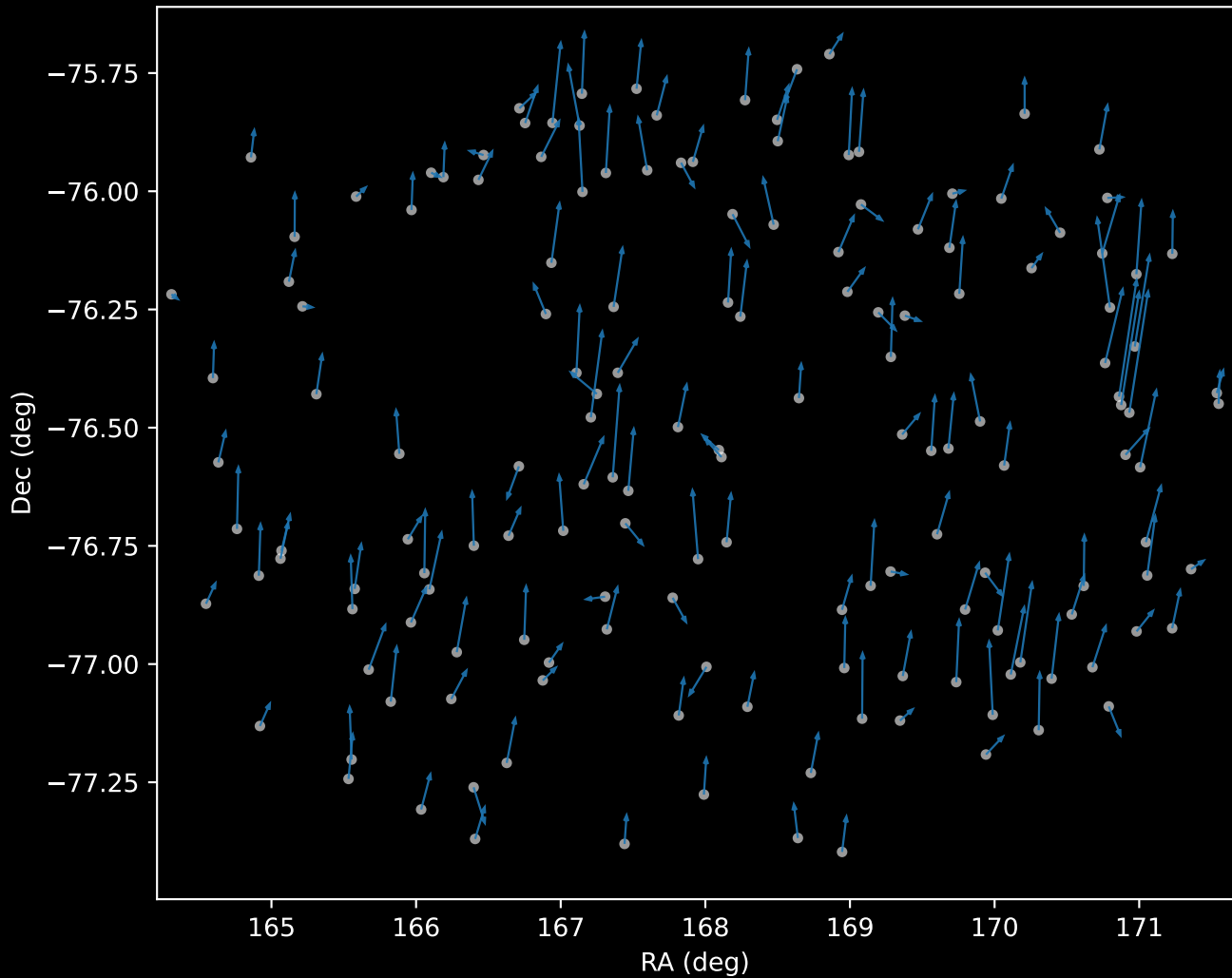
GALAH DR4 Cluster 0 Proper Motion Vectors (n=157)
