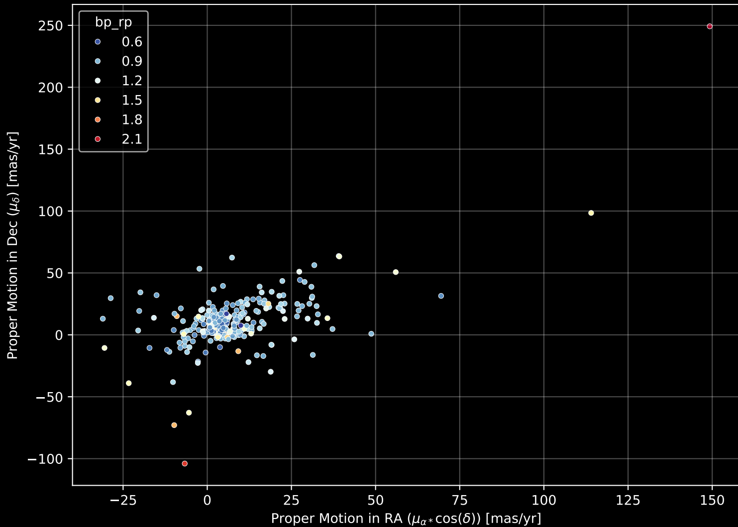
GALAH DR4 Field: [542] Proper Motion Diagram (n= 267)
