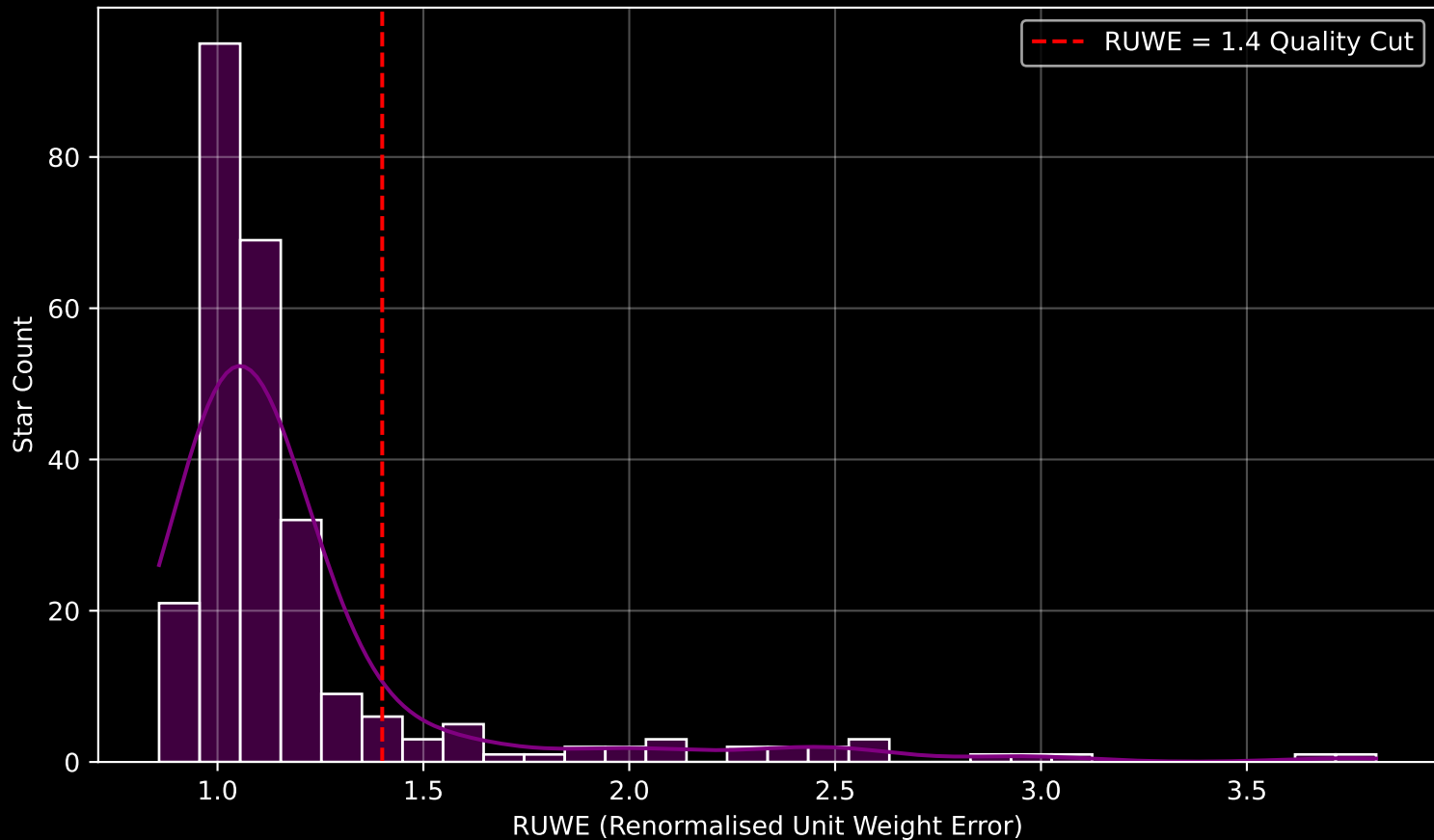
GALAH DR4 Field [542] RUWE Distribution (n= 263)
