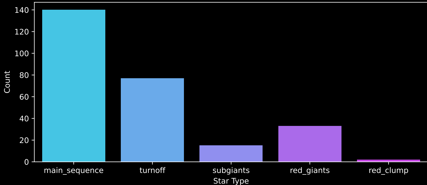
GALAH DR4 Field: [542] Count plot of Star Type
