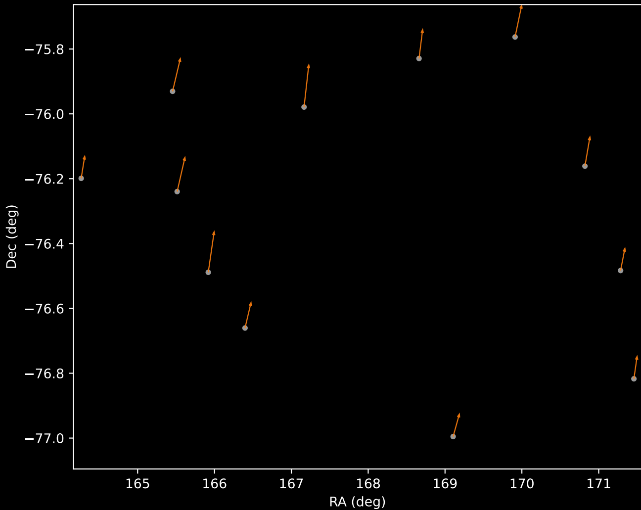
GALAH DR4 Cluster 2 Proper Motion Vectors (n=12)
