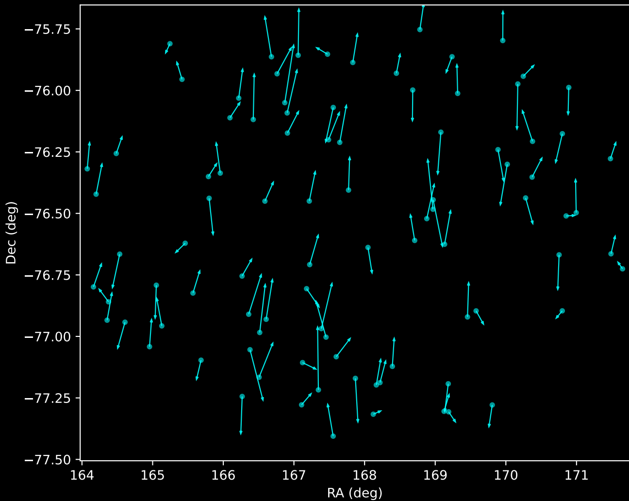
GALAH DR4 Noise Stream Proper Motion Vectors (n=92)
